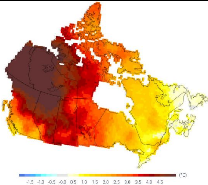
1948 to 2016 Winter Air Temperature Increase
