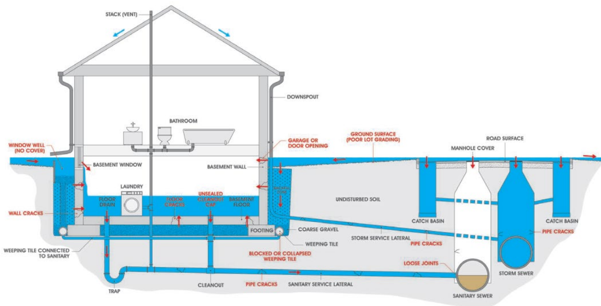
Figure 3.21 Schematic Diagram of Potential Pathways for Basement Flooding from Overland Flow and Storm Sewer Backup (image courtesy of ICLR, 2009)
