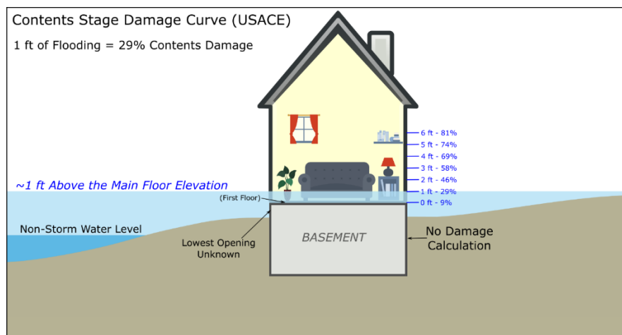
Figure 3.20 Stage Damage Relationship for Contents in a One-Storey Residential Building
