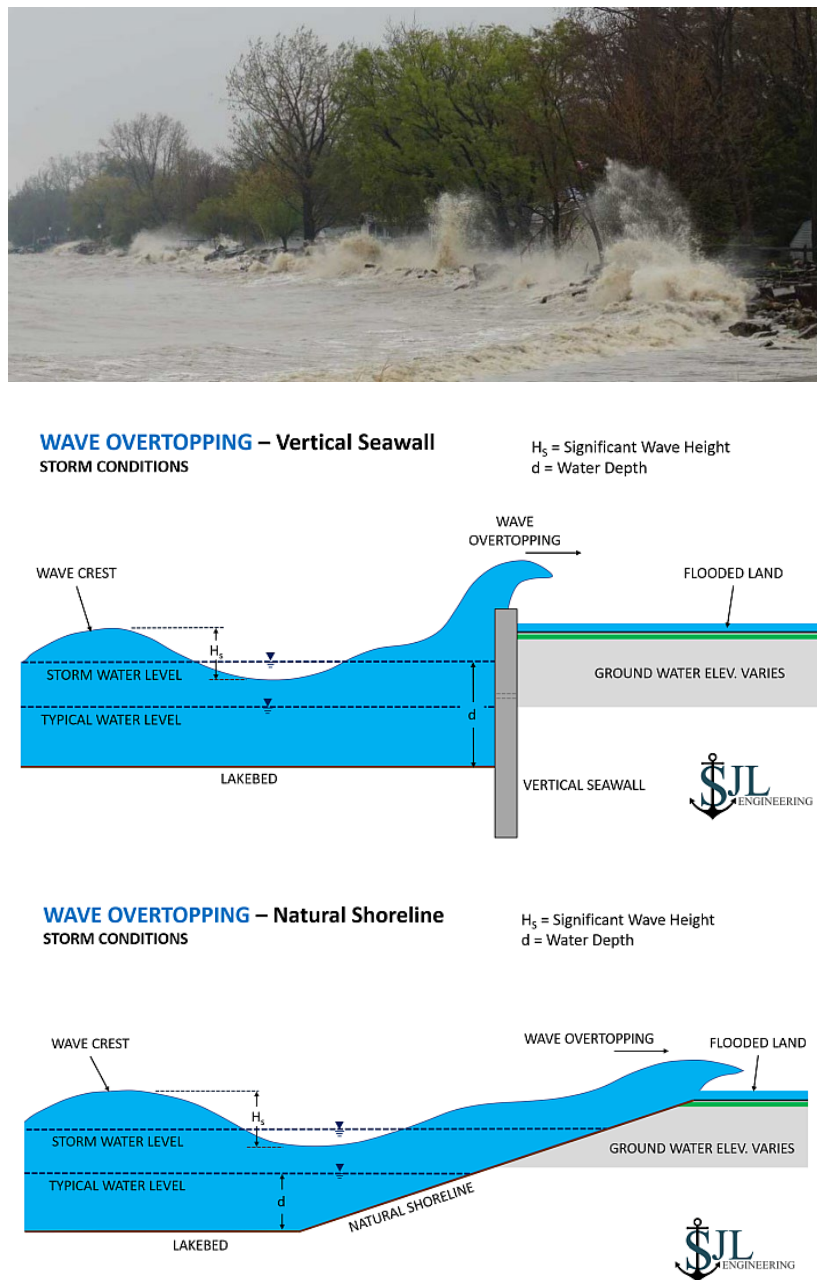
Figure 3.10 Wave Overtopping of Shore Protection Structures and Natural Shorelines
