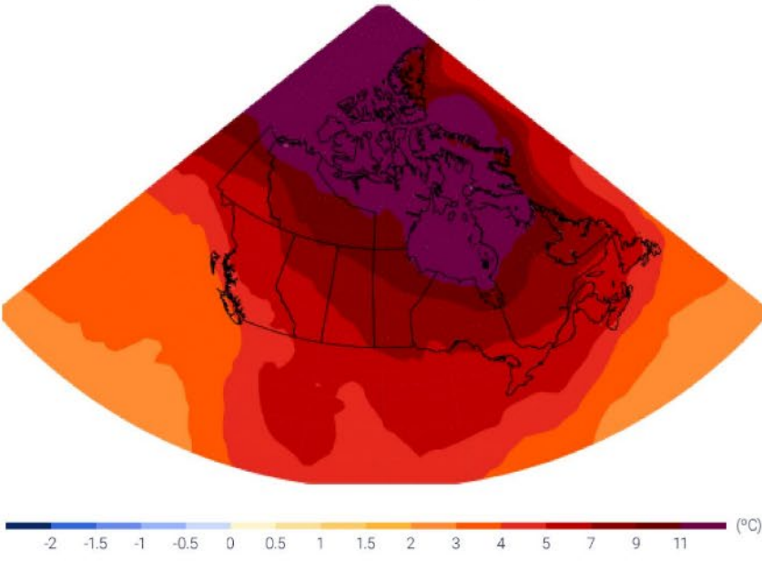
2081-2100 Winter Warming Projection for RCP8.5
