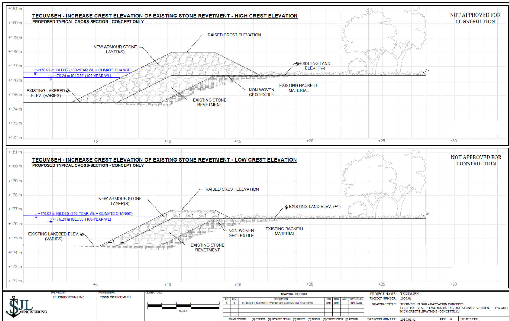
Figure 5.6 Upgrades to Sloping Armour Stone Revetments
